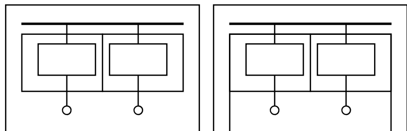
Form 3a No subdivision between terminals and busbars
