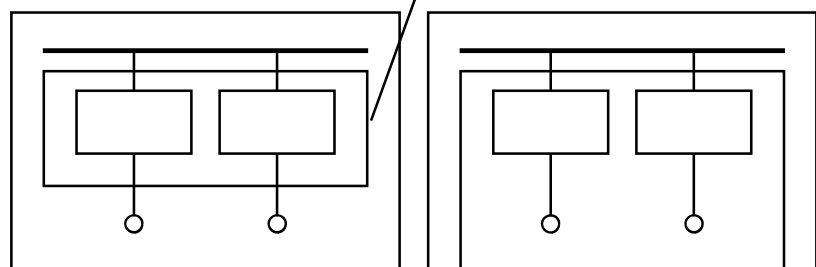
Form 2a No subdivision between terminals and busbars
