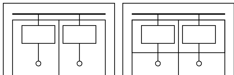
Form 4a Terminals in the same subdivision as the connected functional unit
